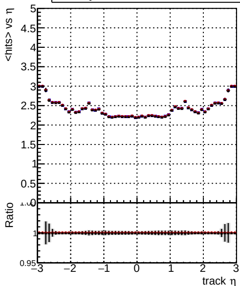
mean hit — DQM_V0001_R000000001_Global_CMSSW_orig — DQM_V0001_R000000001_Global_CMSSW_dt08 — DQM_V0001_R000000001_Global_CMSSW_dt05
