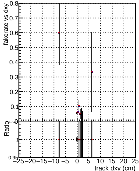
DOM V0001 R0000000001 Global CMSSW orig DOM V0001 R0000000001 Global CMSSW d108
