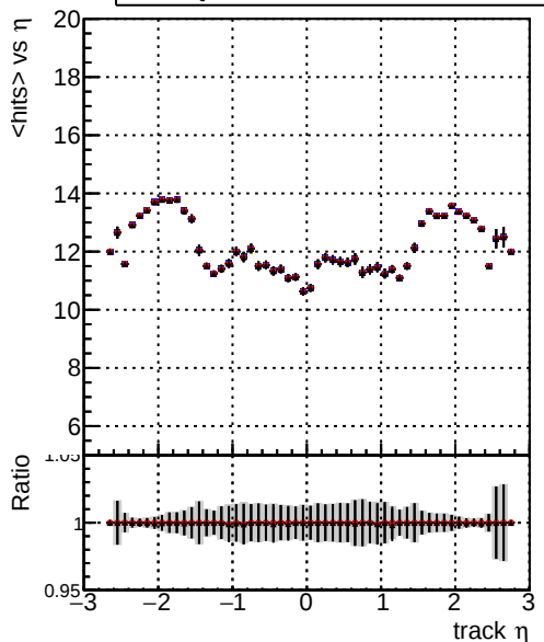
mean hits vs \eta DQM_V0001_R0000000001_Global_CMSSW_orig DQM_V0001_R0000000001_Global_CMSSW_dt08 DQM_V0001_R0000000001_Global_CMSSW_dt05
