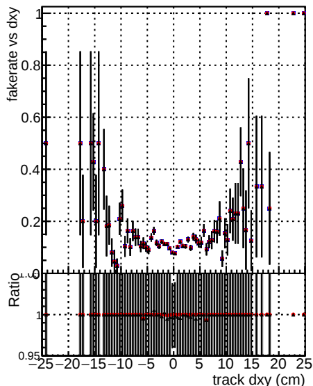
— DOM V0001 R0000000001 Global CMSSW orig — DOM V0001 R0000000001 Global CMSSW d100
