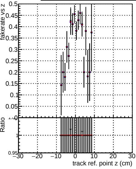
Legend: —●— DQM_V0001_R000000001 Global CMSSW_orig —●— DQM_V0001_R000000001 Global CMSSW_dt08 —●— DQM_V0001_R000000001 Global CMSSW_dt05
