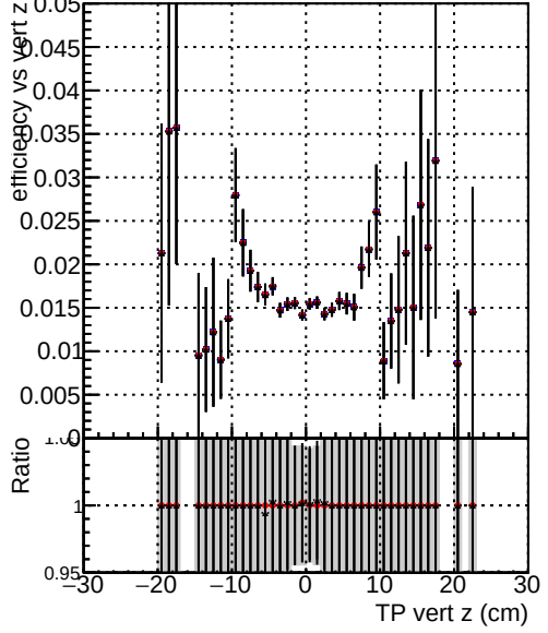
Efficiency vs. sim PV z —●— DQM_V0001_R000000001 Global_CMSSW_orig —●— DQM_V0001_R000000001 Global_CMSSW_dt08 —●— DQM_V0001_R000000001 Global_CMSSW_dt05
