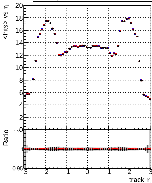
mean hits DQM_V0001_R000000001_Global_CMSSW_orig DQM_V0001_R000000001_Global_CMSSW_dt08 DQM_V0001_R000000001_Global_CMSSW_dt05
