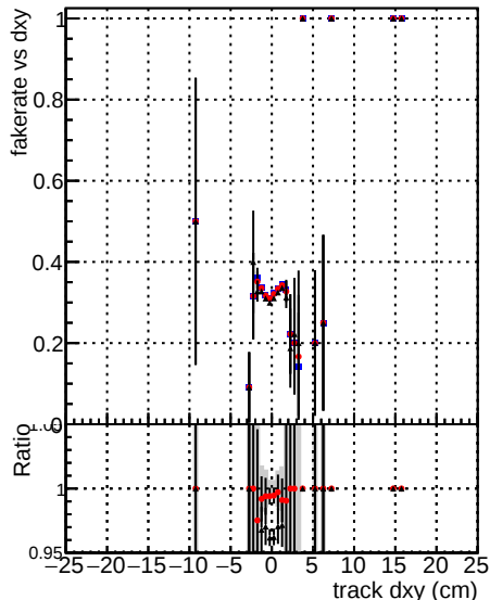
Fake rate vs d —●— DOM V0001 R0000000001 Global CMSSW orig —●— DOM V0001 R0000000001 Global CMSSW d100
