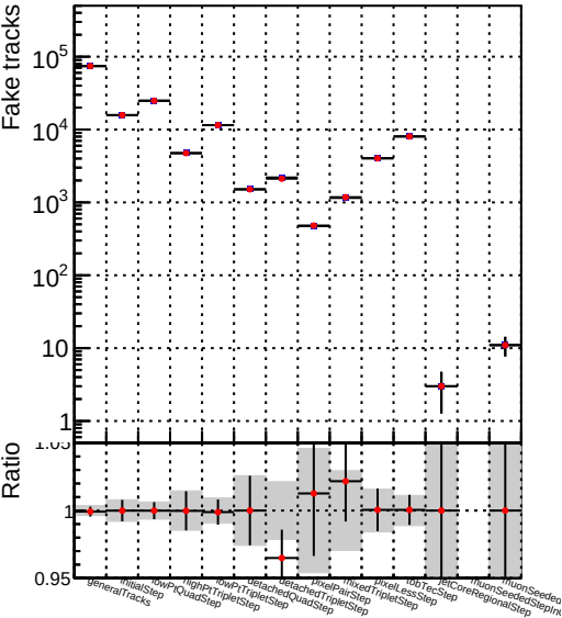
Number —●— DQM_V0001_R000000001_Global_CMSSW_dt05
