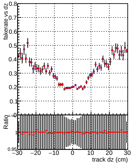
—●— DQM_V0001_R0000000001_Global_CMSSW_dt08 —●— DQM_V0001_R0000000001_Global_CMSSW_dt05
