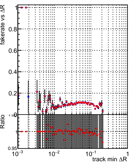
■ DQM_V0001_R000000001_Global_CMSSW_dt08 ■ DQM_V0001_R000000001_Global_CMSSW_dt05
