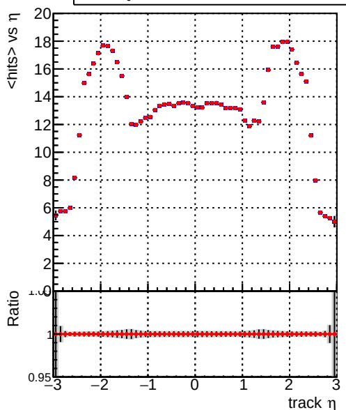
— DQM_V0001_R000000001_Global_CMSSW_dt08 — DQM_V0001_R000000001_Global_CMSSW_dt05
