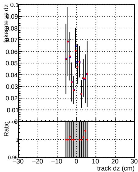
Legend Global CMSSW_dt08 Fake rate vs dz Blue dots DQM V0001_R0000000001 Global Red dots DQM V0001_R0000000001 Global Black line DQM V0001_R0000000001 CMSSW_dt05
