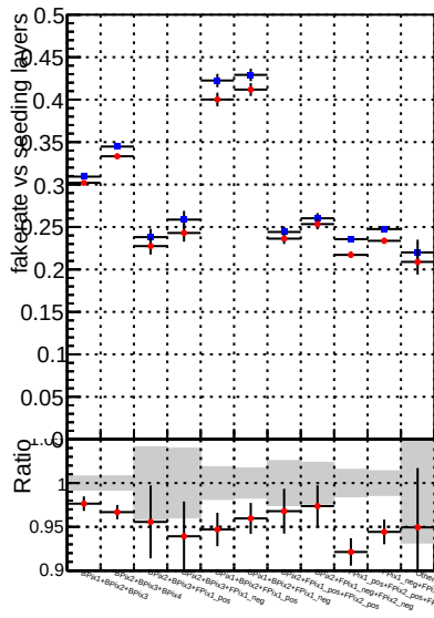
Fake rate vs. —●— DQM V0001_R000000001 Global CMSSW dt08 —●— DQM V0001_R000000001 Global CMSSW dt05
