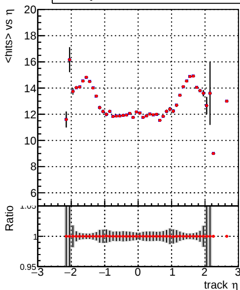
mean hits vs \eta Legend: DQM_V0001_R000000001_Global_CMSSW_dt08 (blue line), DQM_V0001_R000000001_Global_CMSSW_dt05 (red line)
