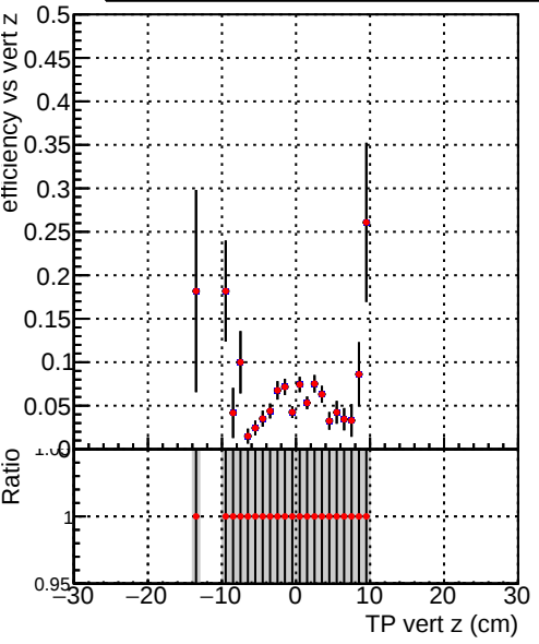
Efficiency vs vert z Legend: DQM_V0001_R000000001_Global_CMSSW_dt08 DQM_V0001_R000000001_Global_CMSSW_dt05
