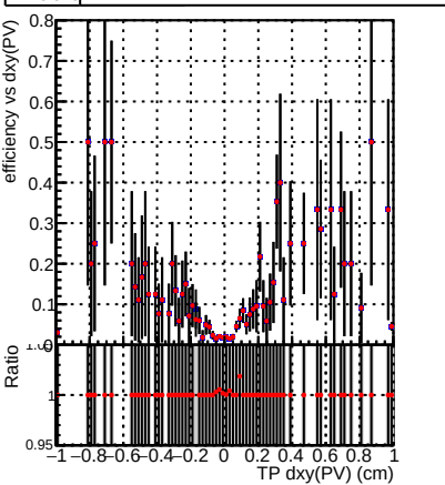
Efficiency vs Dxy(PV)
