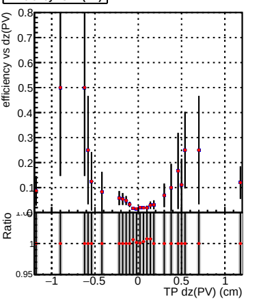
Efficiency vs Dz(PV)
