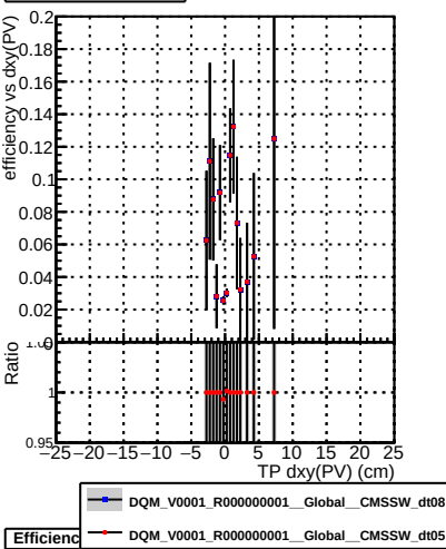
Efficiency vs Dxy(PV)
