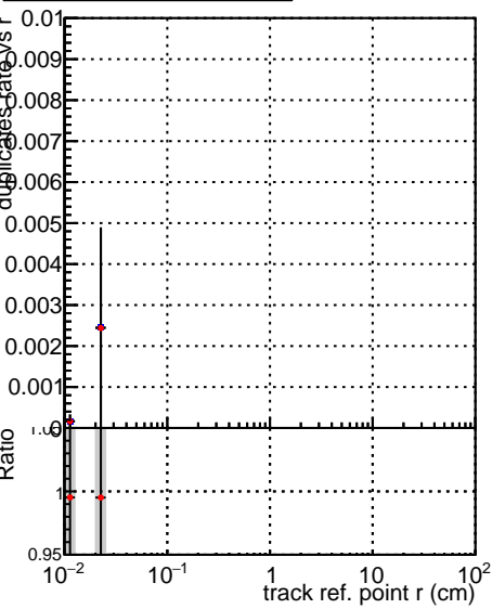
■ DQM_V0001_R000000001_Global_CMSSW_dt08 ● DQM_V0001_R000000001_Global_CMSSW_dt05
