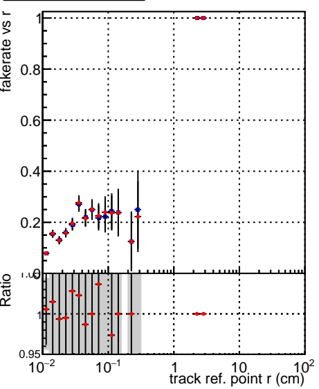
■ DQM_V0001_R000000001_Global_CMSSW_dt08 ● DQM_V0001_R000000001_Global_CMSSW_dt05
