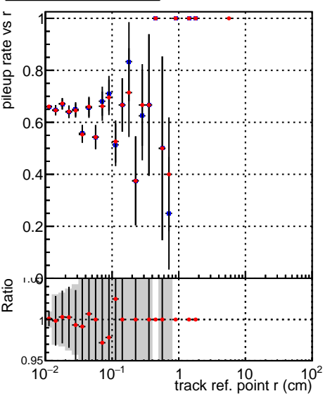
■ DQM_V0001_R000000001_Global_CMSSW_dt08 ● DQM_V0001_R000000001_Global_CMSSW_dt05
