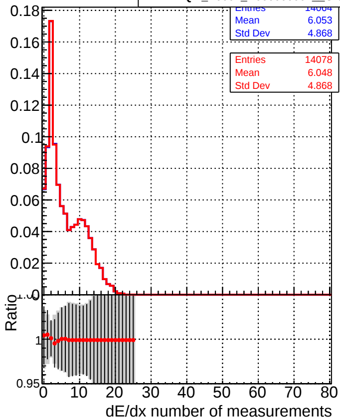
■ DQM_V0001_R000000001_Global_CMSSW_dt08 ● DQM_V0001_R000000001_Global_CMSSW_dt05
