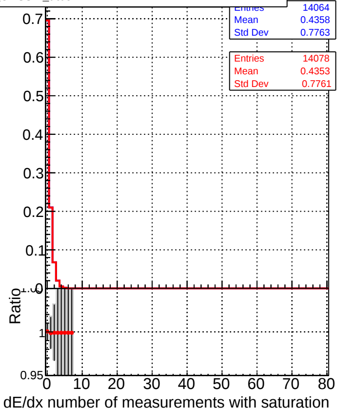
■ DQM_V0001_R000000001_Global_CMSSW_dt08 ● DQM_V0001_R000000001_Global_CMSSW_dt05
