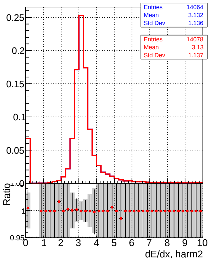
■ DQM_V0001_R000000001_Global_CMSSW_dt08 ● DQM_V0001_R000000001_Global_CMSSW_dt05
