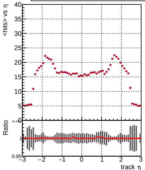
— DQM_V0001_R000000001_Global_CMSSW_dt08 — DQM_V0001_R000000001_Global_CMSSW_dt05
