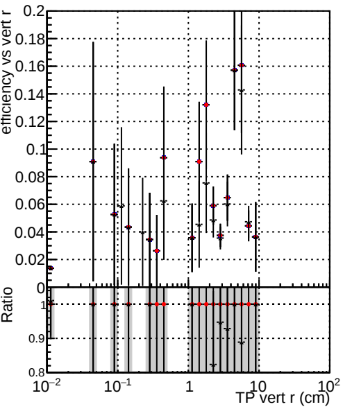
Efficiency vs vertpos Legend: \bullet ./../CMSSW_12_4_0_pre3/src/DQM_V0001_R0000000001_Global_mkFit_batchCAND-adjusted \bullet ./../CMSSW_12_4_0_pre3/src/DQM_V0001_R0000000001_Global_mkFit_CAND \bullet DQM_V0001_R0000000001_Global_mkFit_CAND-AFTERCONFLICT3
