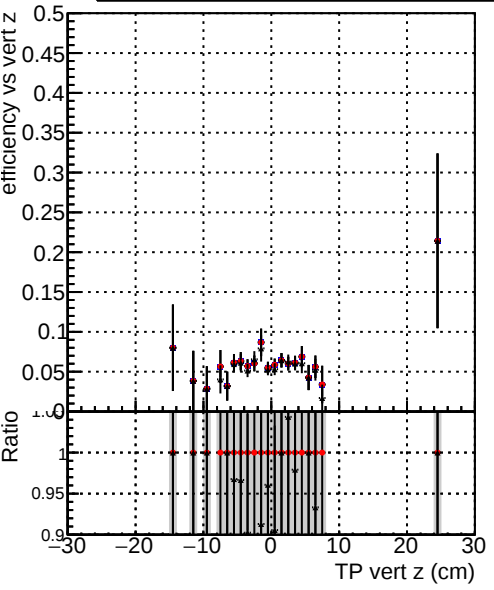
Efficiency vs vert z Legend: Blue line: ./../CMSSW_12_4_0_pre3/src/DQM_V0001_R0000000001_Global_mkFit_batchCAND-adjusted Red line: ./../CMSSW_12_4_0_pre3/src/DQM_V0001_R0000000001_Global_mkFit_CAND Black line: DQM_V0001_R0000000001_Global_mkFit_CAND-AFTERCONFLICT3
