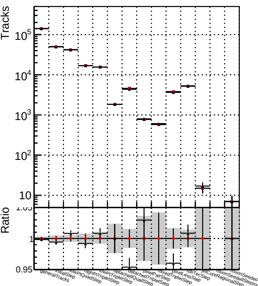
Number Legend ● ../CMSSW_12_4_0_pre3/src/DQM_V0001_R0000000001_Global_mkFit_batchCAND-adjusted ● ../CMSSW_12_4_0_pre3/src/DQM_V0001_R0000000001_Global_mkFit_CAND ● DQM_V0001_R0000000001_Global_mkFit_CAND-AFTERCONFLICT3
