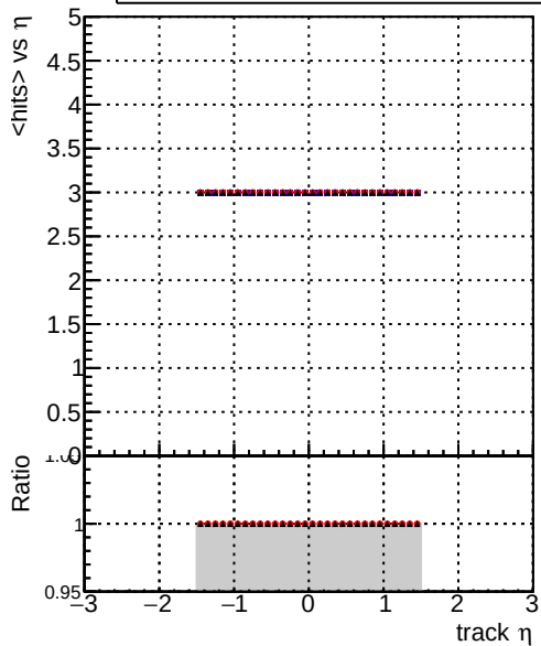
mean hits ./../CMSSW_12_4_0_pre3/src/DQM_V0001_R000000001_Global_mkFit_batchCAND-adjusted ./../CMSSW_12_4_0_pre3/src/DQM_V0001_R000000001_Global_mkFit_CAND DQM_V0001_R000000001_Global_mkFit_CAND-AFTERCONFLICT3
