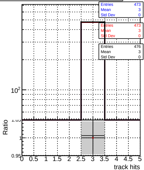
mean hits ./../CMSSW_12_4_0_pre3/src/DQM_V0001_R000000001_Global_mkFit_batchCAND-adjusted ./../CMSSW_12_4_0_pre3/src/DQM_V0001_R000000001_Global_mkFit_CAND DQM_V0001_R000000001_Global_mkFit_CAND-AFTERCONFLICT3
