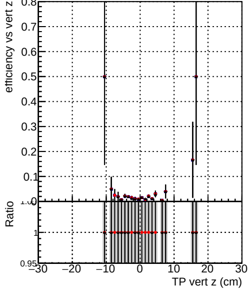
- \bullet ././CMSSW_12_4_0_pre3/src/DQM_V0001_R0000000001_Global_mkFit_batchCAND-adjusted - \bullet ././CMSSW_12_4_0_pre3/src/DQM_V0001_R0000000001_Global_mkFit_CAND - \bullet DQM_V0001_R0000000001_Global_mkFit_CAND-AFTERCONFLICT3
