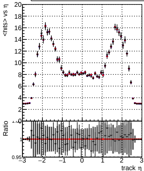
mean hits vs \eta Legend: - Blue line: ./../CMSSW_12_4_0_pre3/src/DQM_V0001_R0000000001_Global_mkFit_batchCAND-adjusted - Red line: ./../CMSSW_12_4_0_pre3/src/DQM_V0001_R0000000001_Global_mkFit_CAND - Black line: DQM_V0001_R0000000001_Global_mkFit_CAND-AFTERCONFLICT3
