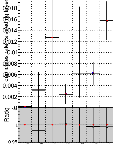
Duplicates rate vs seeding layers
