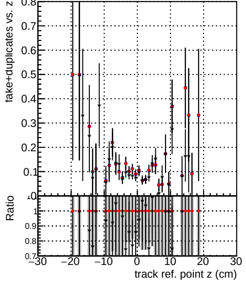
Legend: - Blue line: ./../CMSSW_12_4_0_pre3/src/DQM_V0001_R0000000001_Global_mkFit_batchCAND-adjusted - Red line: ./../CMSSW_12_4_0_pre3/src/DQM_V0001_R0000000001_Global_mkFit_CAND - Black line: DQM_V0001_R0000000001_Global_mkFit_CAND-AFTERCONFLICT3
