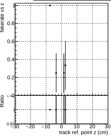
Fake rate vs verpos z
