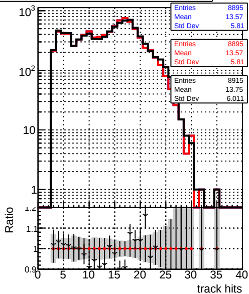
mean hit - - - ./../CMSSW_12_4_0_pre3/src/DQM_V0001_R0000000001_Global_mkFit_batchCAND-adjusted - - - ./../CMSSW_12_4_0_pre3/src/DQM_V0001_R0000000001_Global_mkFit_CAND - - - DQM_V0001_R0000000001_Global_mkFit_CAND-AFTERCONFLICT3
