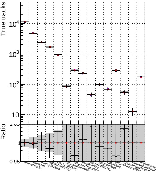
Number Legend: Blue line: ./../CMSSW_12_4_0_pre3/src/DQM_V0001_R0000000001_Global_mkFit_batchCAND-adjusted Red line: ./../CMSSW_12_4_0_pre3/src/DQM_V0001_R0000000001_Global_mkFit_CAND Black line: DQM_V0001_R0000000001_Global_mkFit_CAND-AFTERCONFLICT3
