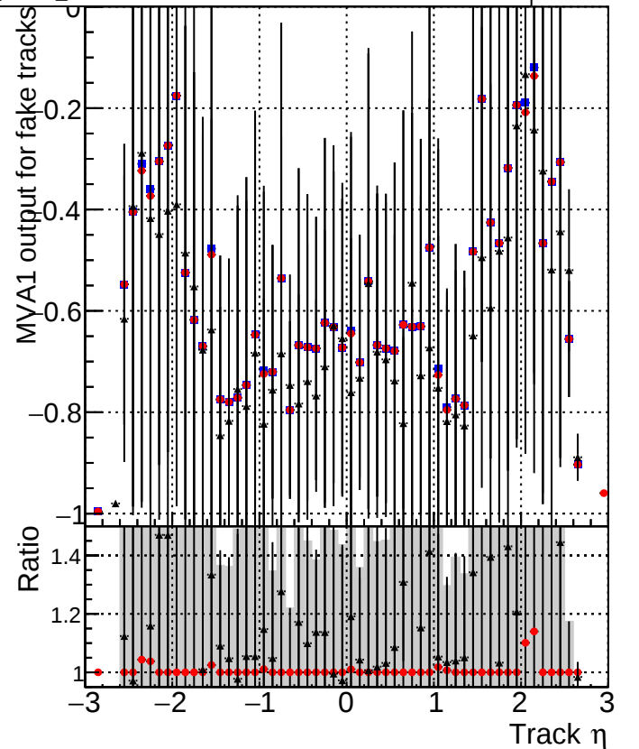
MVA1 of associated tracks (recoToSim) vs. track \eta Legend: Blue square: ../CMSSW_12_4_0_pre3/src/DQM_V0001_R0000000001_Global_mkFit_batchCAND-adjusted Red circle: ../CMSSW_12_4_0_pre3/src/DQM_V0001_R0000000001_Global_mkFit_CAND Black star: DQM_V0001_R0000000001_Global_mkFit_CAND-AFTERCONFLICT3
