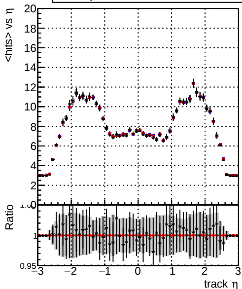
mean hits > \eta Legend: - Blue line: ./../CMSSW_12_4_0_pre3/src/DQM_V0001_R0000000001_Global_mkFit_batchCAND-adjusted - Red line: ./../CMSSW_12_4_0_pre3/src/DQM_V0001_R0000000001_Global_mkFit_CAND - Black line: DQM_V0001_R0000000001_Global_mkFit_CAND-AFTERCONFLICT3
