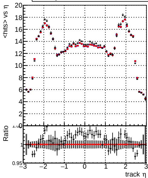
mean hit - - - /J/CMSSW_12_4_0_pre3/src/DQM_V0001_R0000000001_Global_mkFit_batchCAND-adjusted - - - /J/CMSSW_12_4_0_pre3/src/DQM_V0001_R0000000001_Global_mkFit_CAND - - - DQM_V0001_R0000000001_Global_mkFit_CAND-AFTERCONFLICT3
