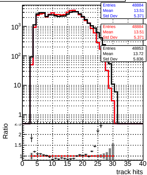
mean hit - - - /J/CMSSW_12_4_0_pre3/src/DQM_V0001_R0000000001_Global_mkFit_batchCAND-adjusted - - - /J/CMSSW_12_4_0_pre3/src/DQM_V0001_R0000000001_Global_mkFit_CAND - - - DQM_V0001_R0000000001_Global_mkFit_CAND-AFTERCONFLICT3
