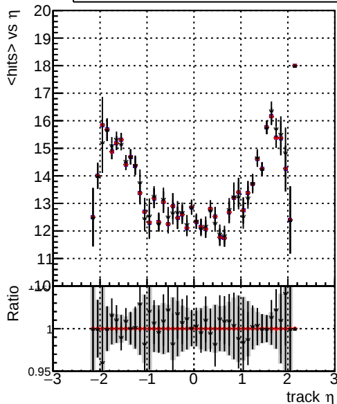
mean hits \frac{1}{N} \sum \langle \text{hits} \rangle vs \eta - \frac{1}{N} \sum \langle \text{hits} \rangle vs \eta (Global mkFit batchCAND-adjusted) - \frac{1}{N} \sum \langle \text{hits} \rangle vs \eta (Global mkFit CAND) - \frac{1}{N} \sum \langle \text{hits} \rangle vs \eta (Global mkFit CAND-AFTERCONFLICT3)
