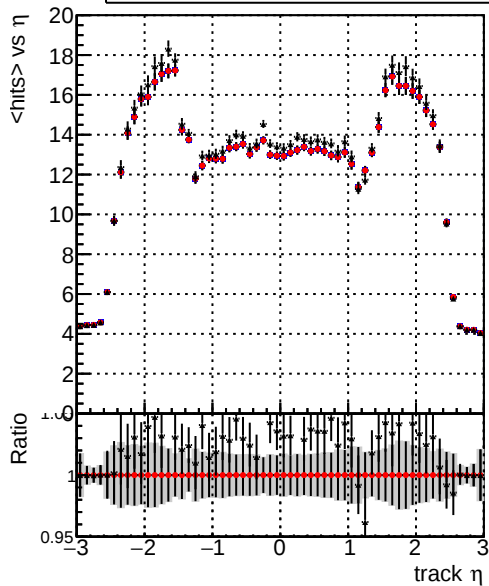
mean hit ././CMSSW_12_4_0_pre3/src/DQM_V0001_R0000000001_Global_mkFit_batchCAND-adjusted ././CMSSW_12_4_0_pre3/src/DQM_V0001_R0000000001_Global_mkFit_CAND DQM_V0001_R0000000001_Global_mkFit_CAND-AFTERCONFLICT3
