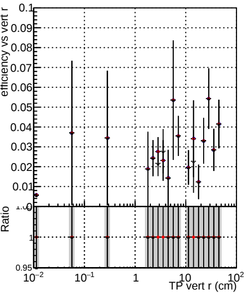
Efficiency vs. TP vert r (cm) Legend: Blue line: ./../CMSSW_12_4_0_pre3/src/DQM_V0001_R0000000001_Global_mkFit_batchCAND-adjusted Red line: ./../CMSSW_12_4_0_pre3/src/DQM_V0001_R0000000001_Global_mkFit_CAND Black line: DQM_V0001_R0000000001_Global_mkFit_CAND-AFTERCONFLICT2
