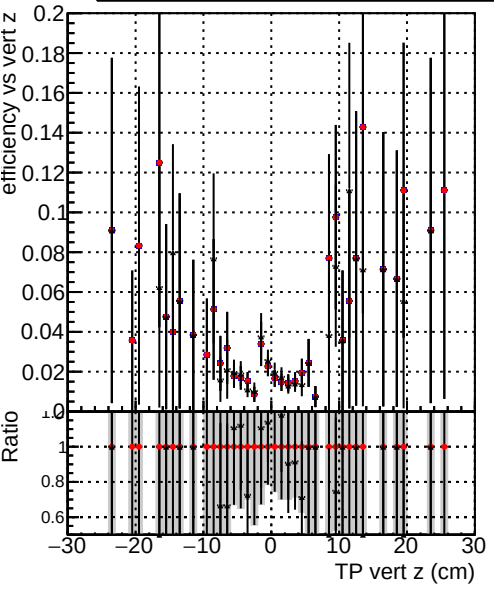
Efficiency vs vertpos Legend: \bullet ././CMSSW_12_4_0_pre3/src/DQM_V0001_R0000000001_Global_mkFit_batchCAND-adjusted \bullet ././CMSSW_12_4_0_pre3/src/DQM_V0001_R0000000001_Global_mkFit_CAND \bullet DQM_V0001_R0000000001_Global_mkFit_CAND-AFTERCONFLICT2
