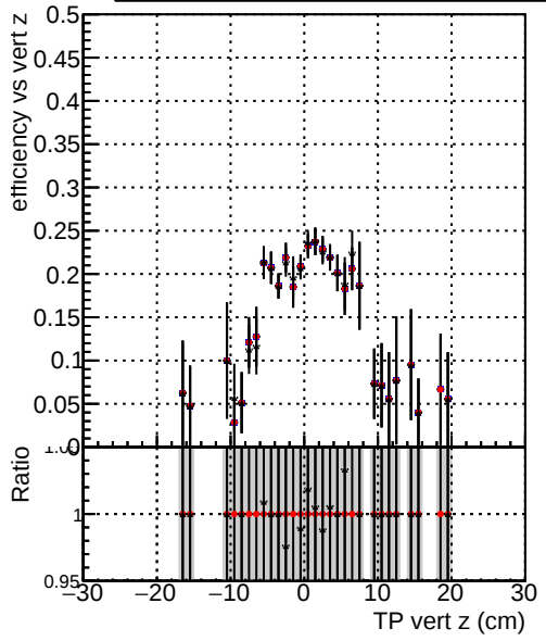
Efficiency vs vert z Legend: ././CMSSW_12_4_0_pre3/src/DQM_V0001_R0000000001_Global_mkFit_batchCAND-adjusted ././CMSSW_12_4_0_pre3/src/DQM_V0001_R0000000001_Global_mkFit_CAND DQM_V0001_R0000000001_Global_mkFit_CAND-AFTERCONFLICT2
