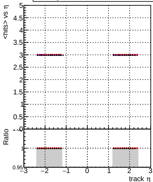
mean hits - - - ././CMSSW_12_4_0_pre3/src/DQM_V0001_R000000001_Global_mkFit_batchCAND-adjusted - - - ././CMSSW_12_4_0_pre3/src/DQM_V0001_R000000001_Global_mkFit_CAND - - - DQM_V0001_R000000001_Global_mkFit_CAND-AFTERCONFLICT2
