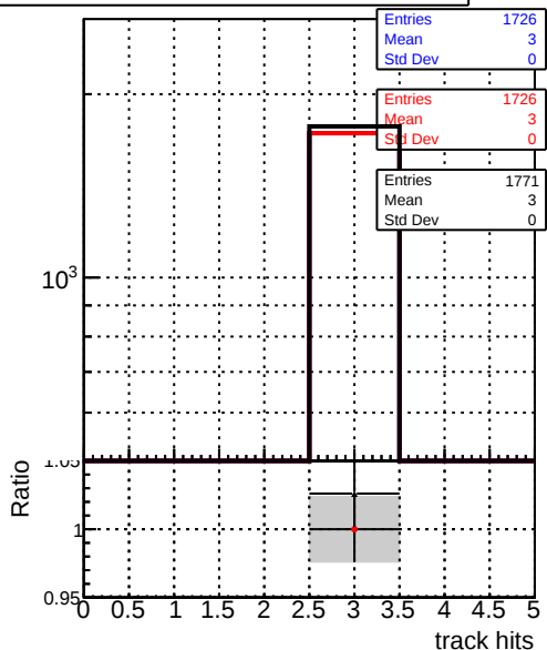
mean hits - - - ././CMSSW_12_4_0_pre3/src/DQM_V0001_R000000001_Global_mkFit_batchCAND-adjusted - - - ././CMSSW_12_4_0_pre3/src/DQM_V0001_R000000001_Global_mkFit_CAND - - - DQM_V0001_R000000001_Global_mkFit_CAND-AFTERCONFLICT2
