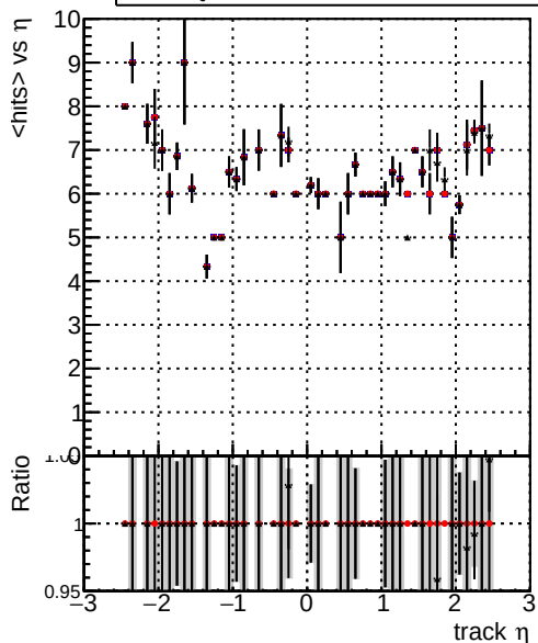
mean hits ././CMSSW_12_4_0_pre3/src/DQM_V0001_R000000001_Global_mkFit_batchCAND-adjusted ././CMSSW_12_4_0_pre3/src/DQM_V0001_R000000001_Global_mkFit_CAND DQM_V0001_R000000001_Global_mkFit_CAND-AFTERCONFLICT2
