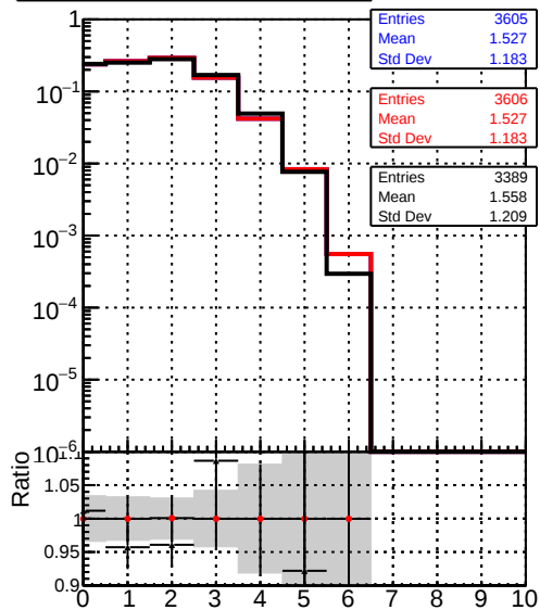
mean hits vs \eta Legend: - Blue line: ./../CMSSW_12_4_0_pre3/src/DQM_V0001_R0000000001_Global_mkFit_batchCAND-adjusted - Red line: ./../CMSSW_12_4_0_pre3/src/DQM_V0001_R0000000001_Global_mkFit_CAND - Black line: DQM_V0001_R0000000001_Global_mkFit_CAND-AFTERCONFLICT2
