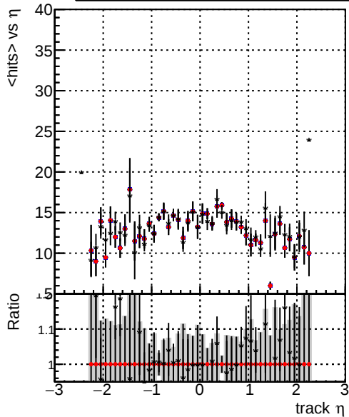
mean hit - - - ././CMSSW_12_4_0_pre3/src/DQM_V0001_R0000000001_Global_mkFit_batchCAND-adjusted - - - ././CMSSW_12_4_0_pre3/src/DQM_V0001_R0000000001_Global_mkFit_CAND - - - DQM_V0001_R0000000001_Global_mkFit_CAND-AFTERCONFLICT2
