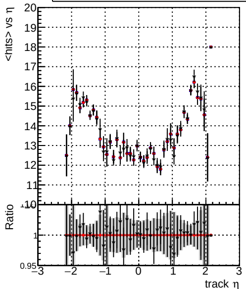
mean hits vs \eta - - - Global_mkFit_batchCAND-adjusted - - - Global_mkFit_CAND - - - DQM_V0001_R000000001_Global_mkFit_CAND-AFTERCONFLICT2
