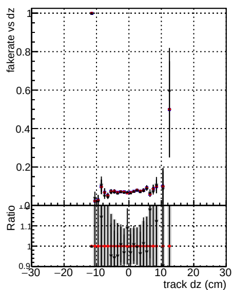
Fake rate vs dz - - - /CMSSW_12_4_0_pre3/src/DOCV0001_R000000001_Global_mkFit_batchCAND-adjusted - - - /CMSSW_12_4_0_pre3/src/DOCV0001_R000000001_Global_mkFit_CAND - - - DOCV0001_R000000001_Global_mkFit_CAND-AFTERCONFLICT2
