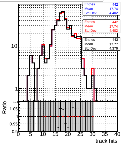
mean hits Global_mkFit_batchCAND-adjusted Global_mkFit_CAND DQM_V0001_R000000001_Global_mkFit_CAND-AFTERCONFLICT2
