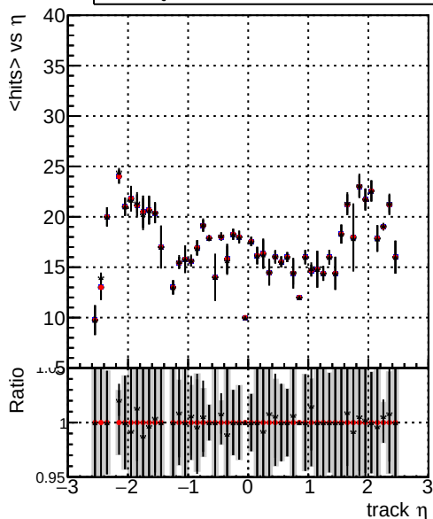
mean hits Global_mkFit_batchCAND-adjusted Global_mkFit_CAND DQM_V0001_R000000001_Global_mkFit_CAND-AFTERCONFLICT2
