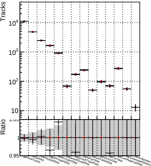
Number Series Color Symbol Path Global mkFit Batch Adjusted 1 Blue Circle ./../CMSSW_12_4_0_pre3/src/DQM_V0001_R0000000001 Global mkFit batch CAND-adjusted 2 Red Circle ./../CMSSW_12_4_0_pre3/src/DQM_V0001_R0000000001 Global mkFit CAND 3 Black Circle ./../CMSSW_12_4_0_pre3/src/DQM_V0001_R0000000001 Global mkFit CAND AFTERCONFLICT2
