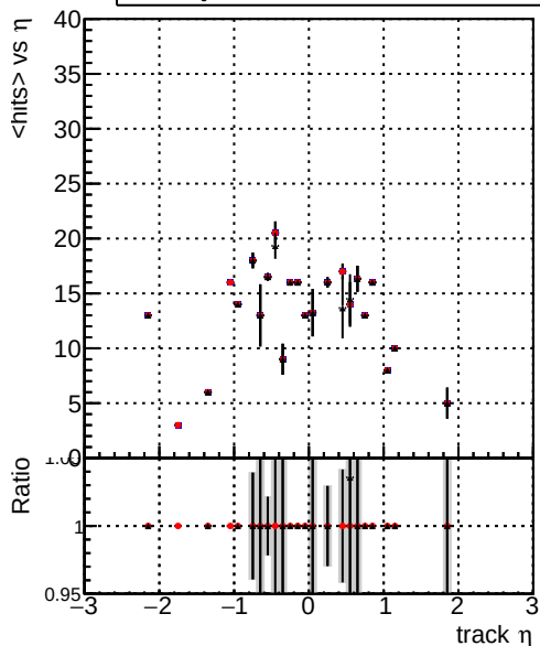
mean hits \frac{1}{N} \sum \text{hits} vs \eta - \frac{1}{N} \sum \text{hits} vs \eta (Global mkFit batchCAND-adjusted) - \frac{1}{N} \sum \text{hits} vs \eta (Global mkFit CAND) - \frac{1}{N} \sum \text{hits} vs \eta (Global mkFit CAND-AFTERCONFLICT2)
