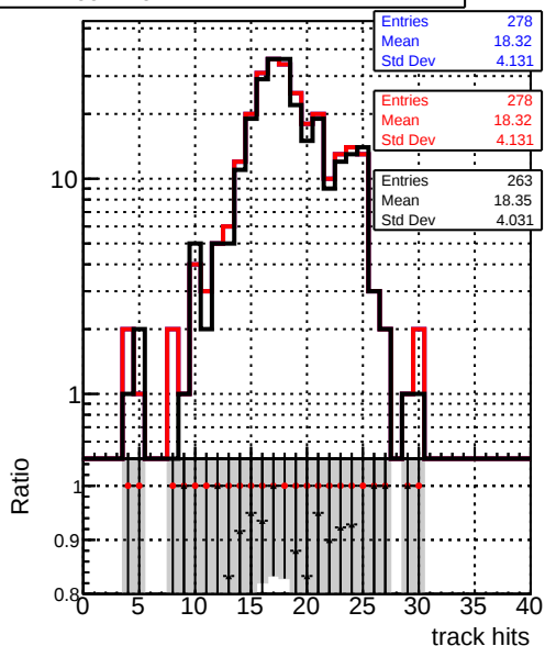
mean hit Global_mkFit_batchCAND-adjusted Global_mkFit_CAND Global_mkFit_CAND-AFTERCONFLICT2
