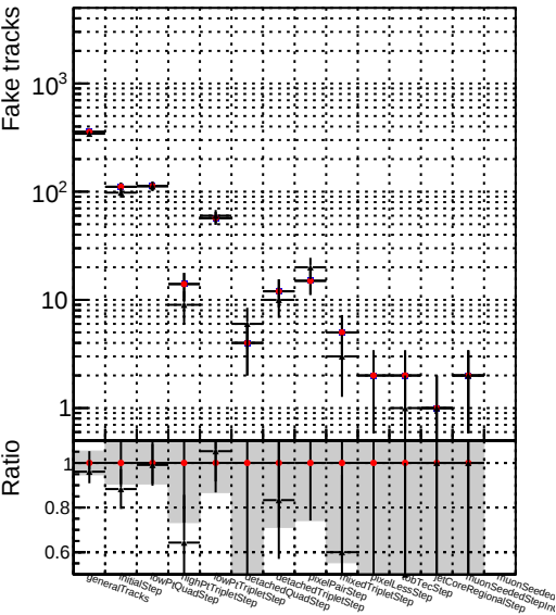
Number — DQM_V0001_R000000001_Global_mkFit_CAND-AFTERCONFLICT2
