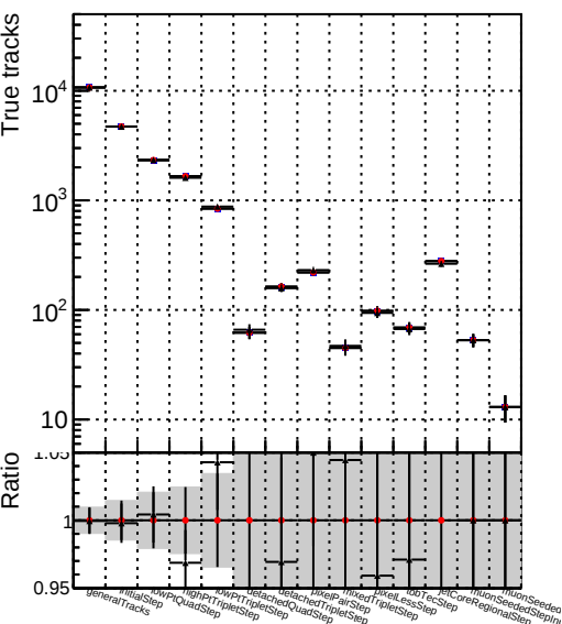
- .../CMSSW_12_4_0_pre3/src/DQM_V0001_R000000001_Global_mkFit_batchCAND-adjusted
